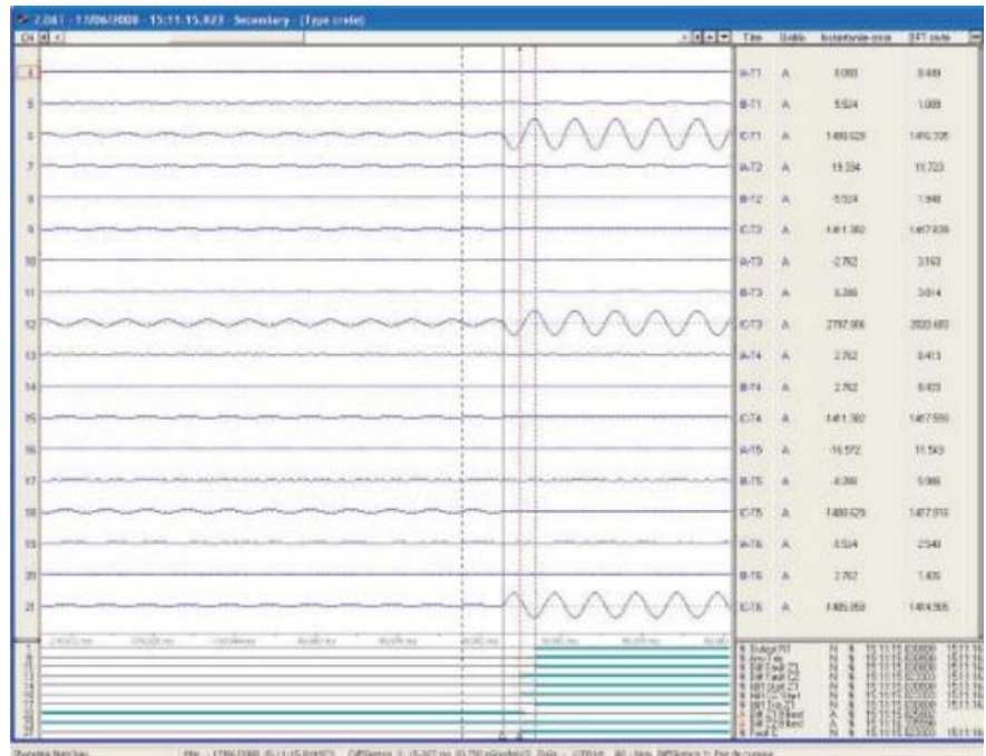
Disturbance record viewed in S1
