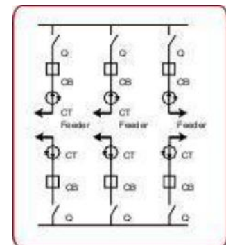
Topology scheme examples
