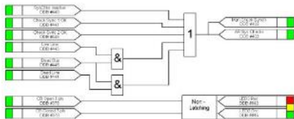
Programmable scheme logic editor (MiCOM Grid Solutions S1 Agile)
