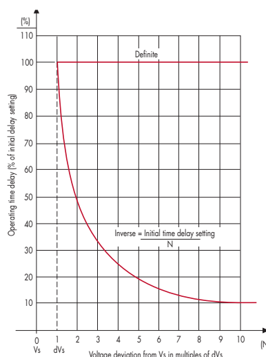
Fig 1 Operating time characteristics
