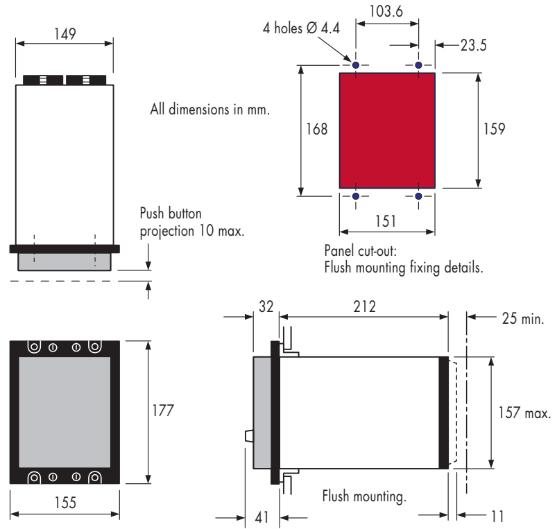
Figure 3 Case outline 30TE (size 6)
